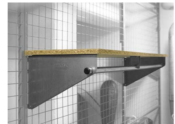
FLEXIBLE CHIPBOARD SHELF WITH BRACKETS
