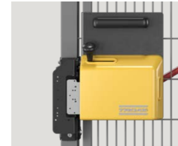
SAFE LOCK Fits all door variants and can be equipped with the safety switch of your choice.
