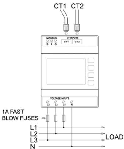
3 Phase, 4 wire
