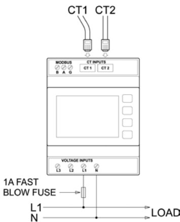
Single Phase, 2 wire
