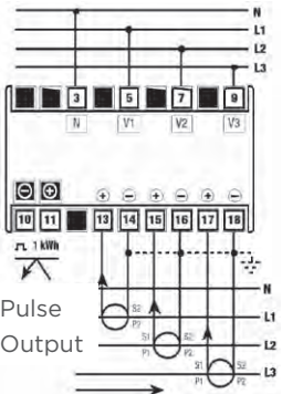
DRK-3PCT Three-phase CT connected 5A(*) four-wire system
