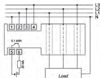
Four-wire System
