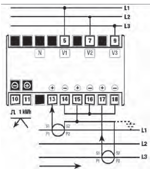
DRK-3PCT Three-phase CT connected 5A(*) three-wire system
