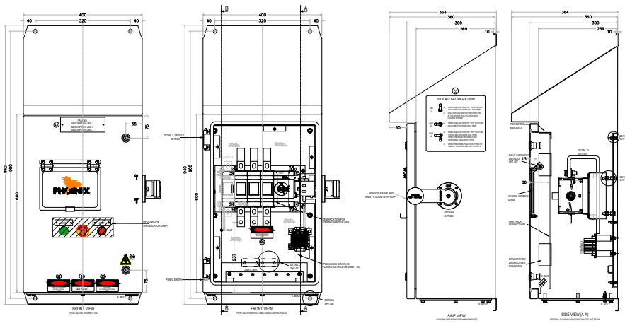
Rear Busbar Connection System
